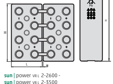
Fig. F Series OPzV
